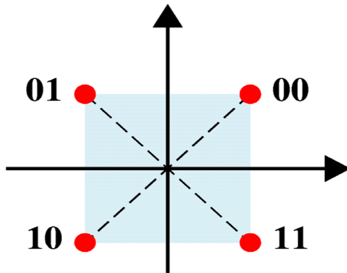
4-QAM
