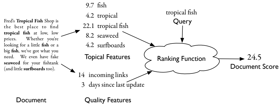
Fig. 5.1. The components of the abstract model of ranking: documents, features, queries, the retrieval function, and document scores
