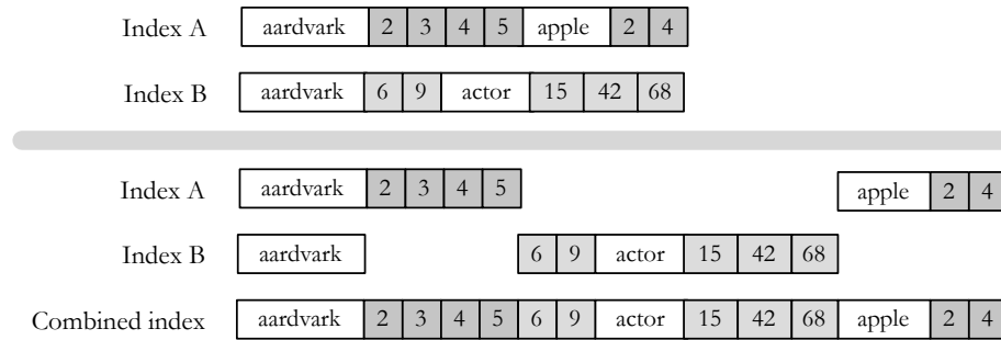
Fig. 5.9. An example of index merging. The first and second indexes are merged together to produce the combined index.
