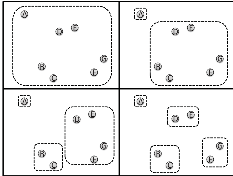
Fig. 9.11. Example of divisive clustering with K = 4 . The clustering proceeds from left to right and top to bottom, resulting in four clusters.
