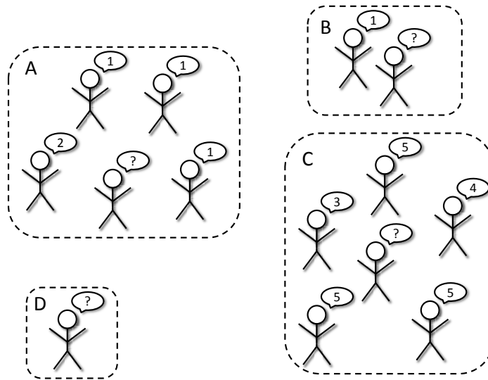
Fig. 10.9. Illustration of collaborative filtering using clustering. Groups of similar users are outlined with dashed lines. Users and their ratings for some item are given. In each group, there is a single user who has not judged the item. For these users, the unjudged item is assigned an automatic rating based on the ratings of similar users.
