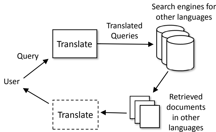
Fig. 6.9. Cross-language search
