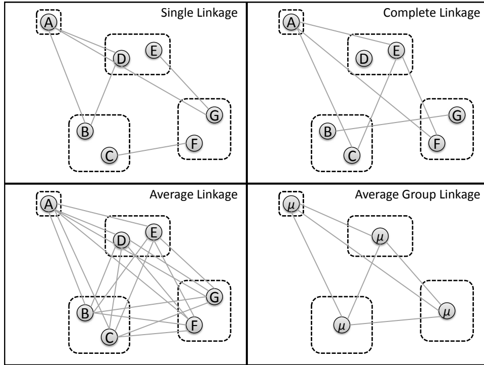
Fig. 9.15. Illustration of how various clustering cost functions are computed
