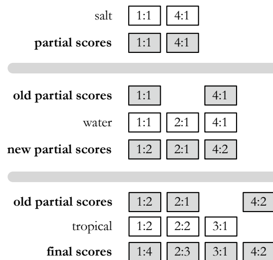
Fig. 5.17. Term-at-a-time query evaluation
