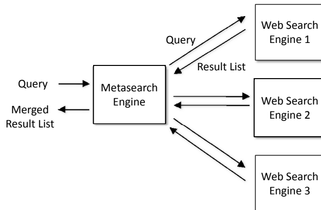
Fig. 10.10. Metasearch engine architecture. The query is broadcast to multiple web search engines and result lists are merged.
