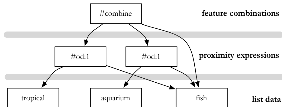
Fig. 5.23. Evaluation tree for the structured query #combine(#od:1(tropical fish) #od:1(aquarium fish) fish)
