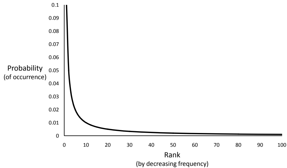
Fig. 4.1. Rank versus probability of occurrence for words assuming Zipf's law ( \text{rank} \times \text{probability} = 0.1 )
