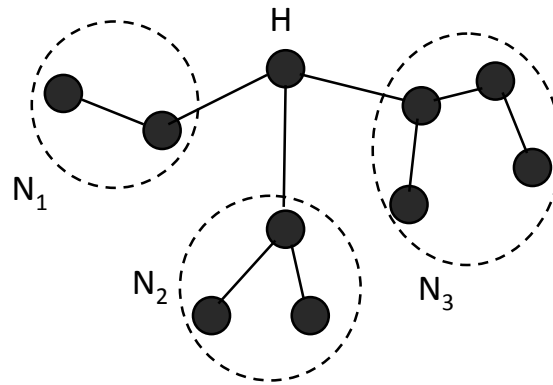
Fig. 10.12. Neighborhoods ( N_i ) of a hub node ( H ) in a hierarchical P2P network
