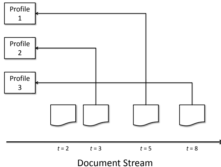
Fig. 10.6. Example of a static filtering system. Documents arrive over time and are compared against each profile. Arrows from documents to profiles indicate the document matches the profile and is retrieved.
