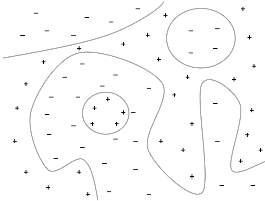
Fig. 9.6. Example data set where non-parametric learning algorithms, such as a nearest neighbor classifier, may outperform parametric algorithms. The pluses and minuses indicate positive and negative training examples, respectively. The solid gray line shows the actual decision boundary, which is highly non-linear.
