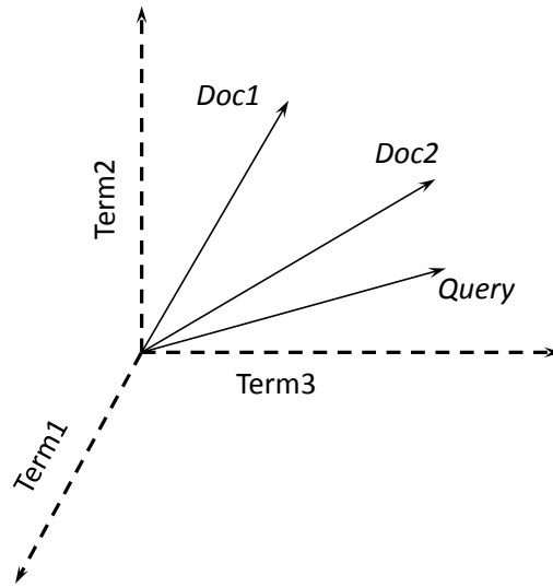
Fig. 7.2. Vector representation of documents and queries
