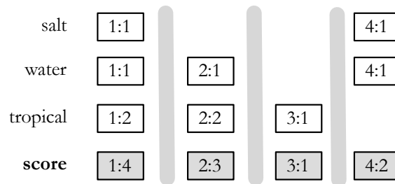
Fig. 5.15. Document-at-a-time query evaluation. The numbers (x:y) represent a document number (x) and a word count (y) .
