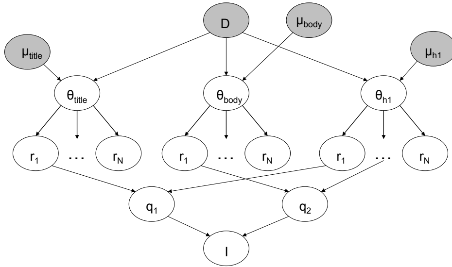
Fig. 7.4. Example inference network model
