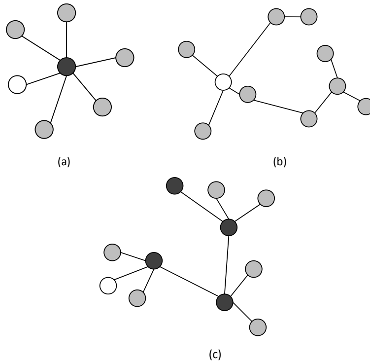
Fig. 10.11. Network architectures for distributed search: (a) central hub; (b) pure P2P; and (c) hierarchical P2P. Dark circles are hub or superpeer nodes, gray circles are provider nodes, and white circles are consumer nodes.
