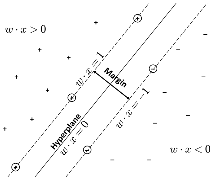
Fig. 9.4. Graphical illustration of Support Vector Machines for the linearly separable case. Here, the hyperplane defined by w is shown, as well as the margin, the decision regions, and the support vectors, which are indicated by circles.
