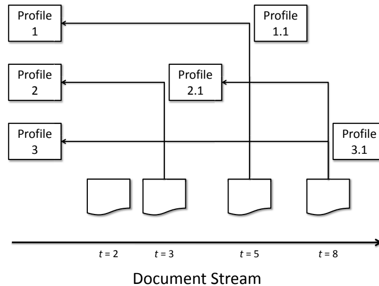
Fig. 10.7. Example of an adaptive filtering system. Documents arrive over time and are compared against each profile. Arrows from documents to profiles indicate the document matches the profile and is retrieved. Unlike static filtering, where profiles are static over time, profiles are updated dynamically (e.g., when a new match occurs).
