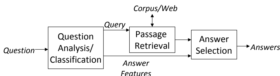
Fig. 11.5. Question answering system architecture
