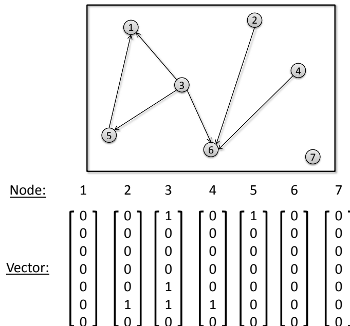
Fig. 10.4. Example of how nodes within a directed graph can be represented as vectors. For a given node p , its vector representation has component q set to 1 if p \rightarrow q .
