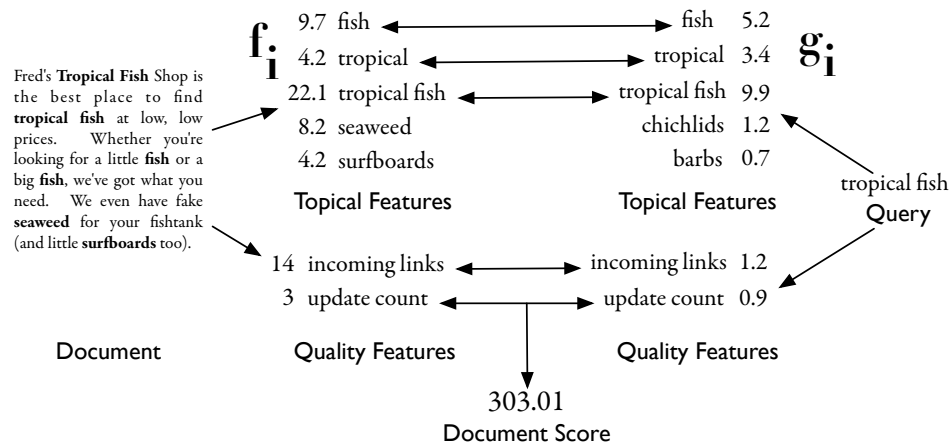
Fig. 5.2. A more concrete model of ranking. Notice how both the query and the document have feature functions in this model.
