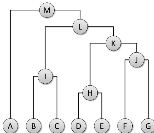
Fig. 9.12. Example of agglomerative clustering with K = 4 . The clustering proceeds from left to right and top to bottom, resulting in four clusters.
