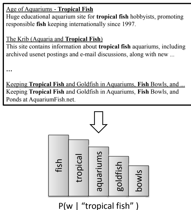
Fig. 10.1. Search results used to enrich a tag representation. In this example, the tag being expanded is “tropical fish”. The query “tropical fish” is run against a search engine, and the snippets returned are then used to generate a distribution over related terms.
