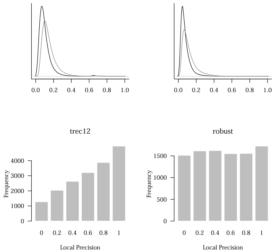
Fig. 9.18. Cluster hypothesis tests on two TREC collections. The top two compare the distributions of similarity values between relevant-relevant and relevant-nonrelevant pairs (light gray) of documents. The bottom two show the local precision of the relevant documents.
