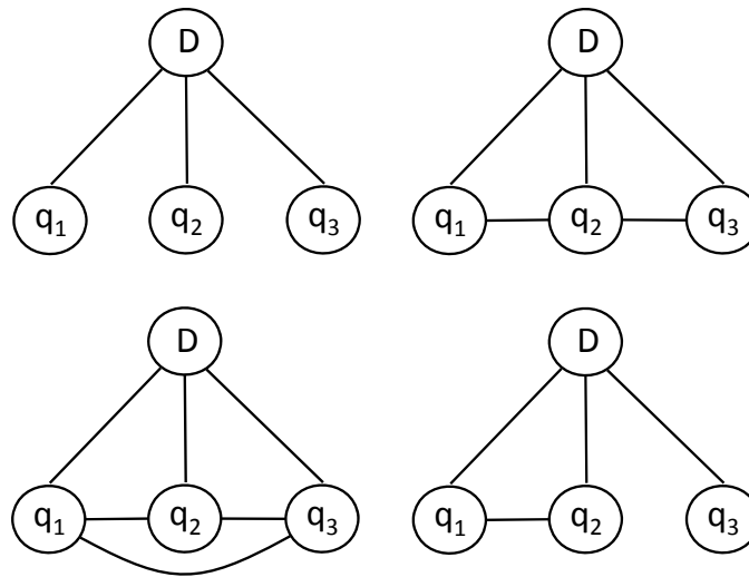
Fig. 11.1. Example Markov Random Field model assumptions, including full independence (top left), sequential dependence (top right), full dependence (bottom left), and general dependence (bottom right)
