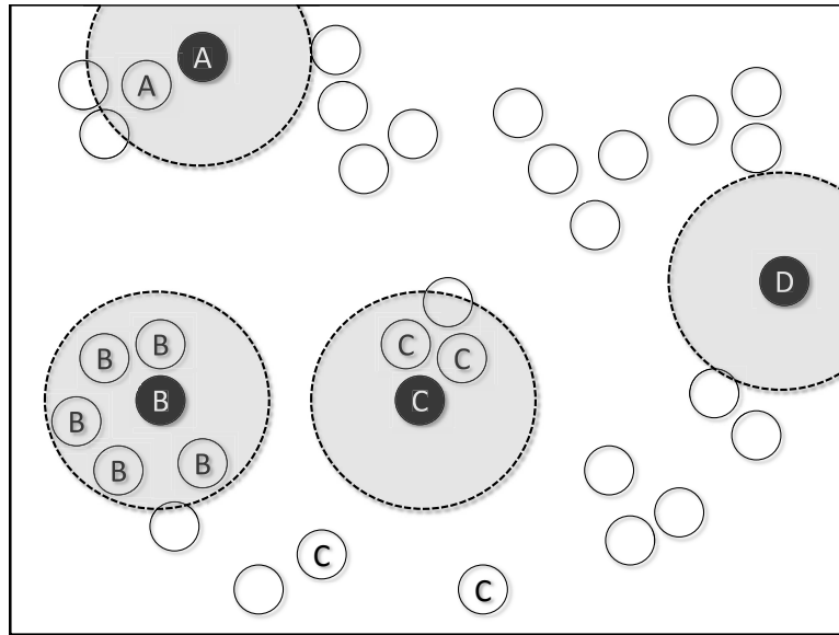
Fig. 9.17. Example of overlapping clustering using Parzen windows. The clusters for the black points (A, B, C, and D) are shown. The shaded circles indicate the windows used to determine cluster membership. The neighbors for each black point are shaded gray and labeled accordingly.
