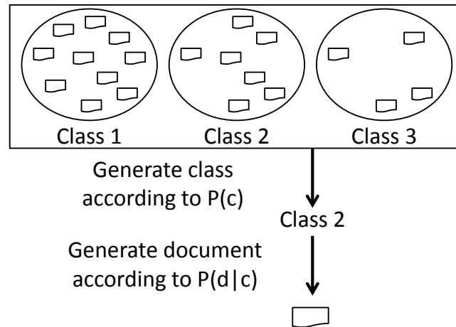
Fig. 9.5. Generative process used by the Naïve Bayes model. First, a class is chosen according to P(c) , and then a document is chosen according to P(d|c) .
