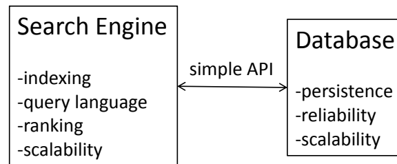
Fig. 11.3. Functions provided by a search engine interacting with a simple database system
