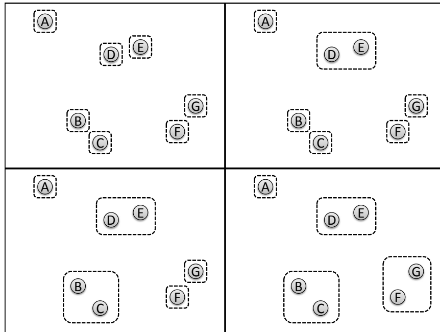
Fig. 9.12. Example of agglomerative clustering with K = 4 . The clustering proceeds from left to right and top to bottom, resulting in four clusters.
