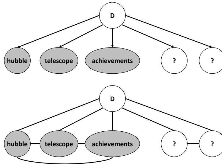
Fig. 11.2. Graphical model representations of the relevance model technique (top) and latent concept expansion (bottom) used for pseudo-relevance feedback with the query “hubble telescope achievements”
