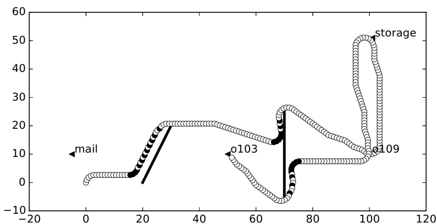
Figure 2.9: A simulation of the robot carrying out the plan of Example 2.6 (page 63). The black lines are obstacles. The robot starts at position (0,0) and follows the trajectory of the overlapping circles; the filled circles are when the whisker sensor is on. The robot goes to o109, storage, o109, and o103 in turn
