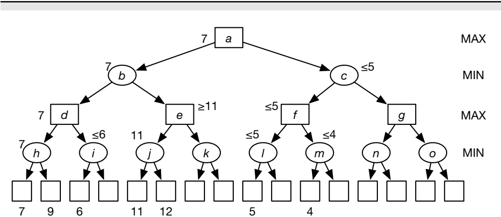
Figure 14.6: A zero-sum game tree showing which nodes can be pruned
