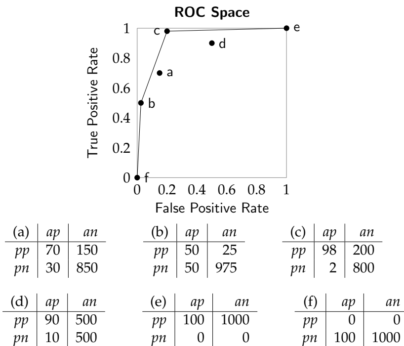
Figure 7.7: Six predictors in the ROC space
