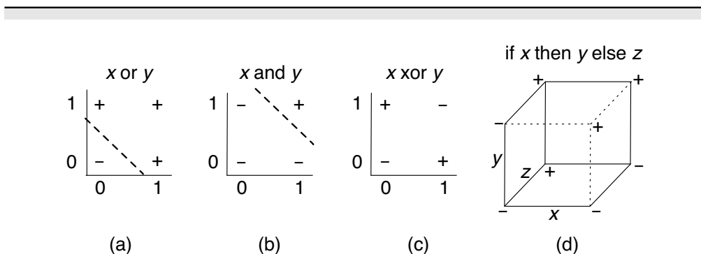
Figure 7.13: Linear separators for Boolean functions
