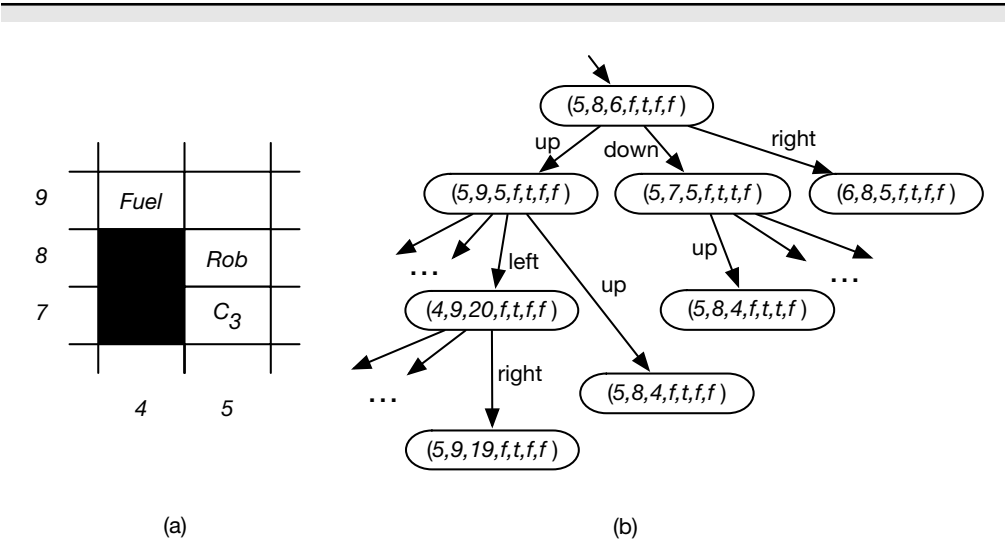
Figure 3.2: Part of the video game and state space of Example 3.3
