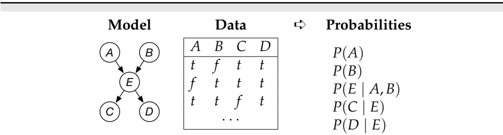
Figure 10.9: Deriving probabilities with a hidden variable
