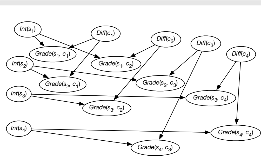
Figure 17.5: A grounding that is sufficient to predict from the data in Figure 17.3. Instances of Grade(S, C) that are not observed or queried do not need to be created.
