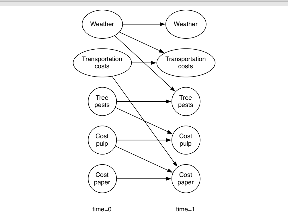
Figure 9.20: Two-stage dynamic belief network for paper pricing
