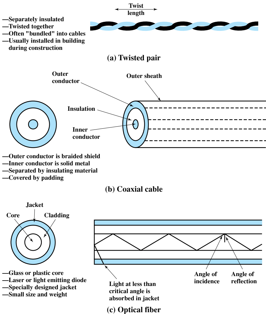
Figure 4.2 Guided Transmission Media
