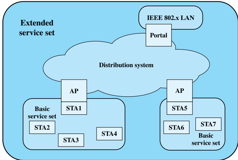
Figure 17.4 IEEE 802.11 Architecture
