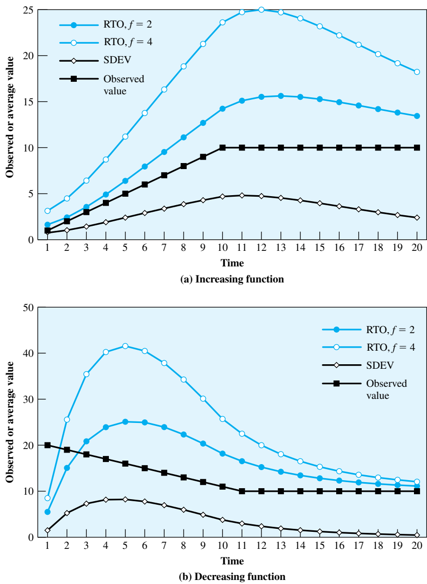
Figure 20.12 Jacobson's RTO Calculation
