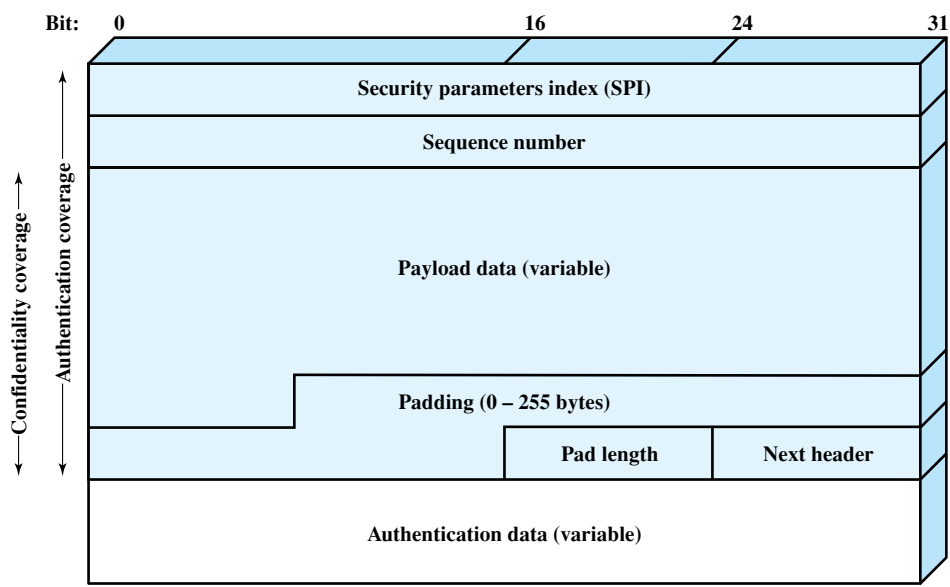
Figure 21.17 IPsec ESP Format
