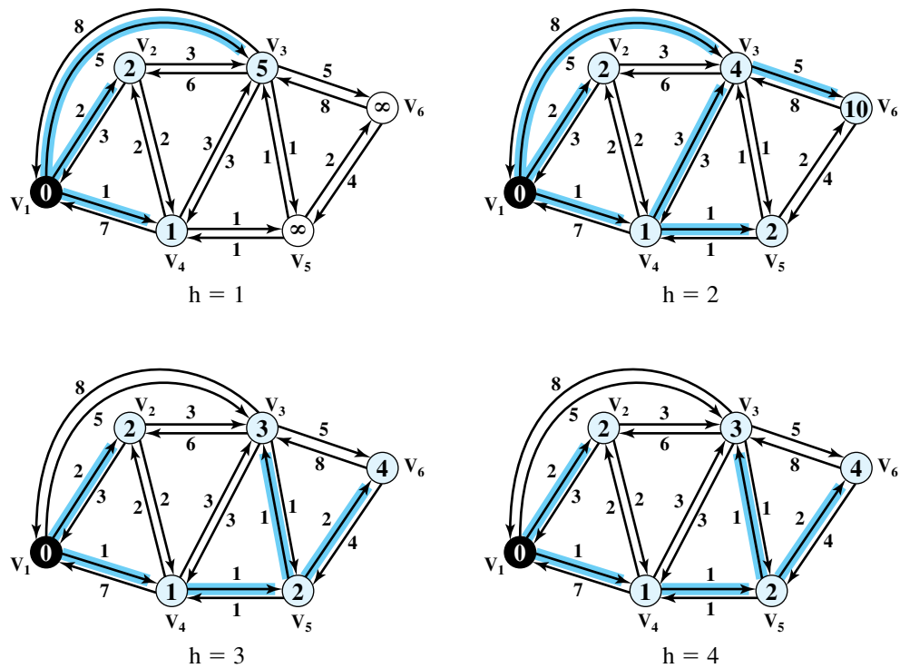
Figure 12.10 Bellman-Ford Algorithm Applied to Graph of Figure 12.1
