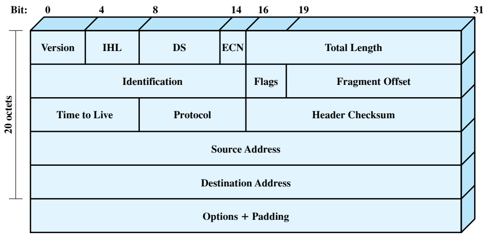
Figure 18.6 IPv4 Header
