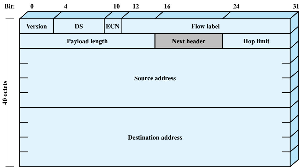
(b) IPv6 header
