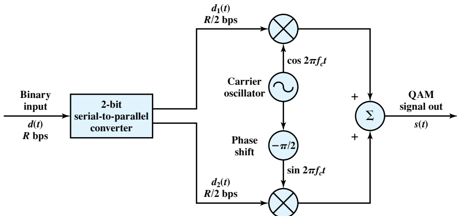
Figure 5.14 QAM Modulator
