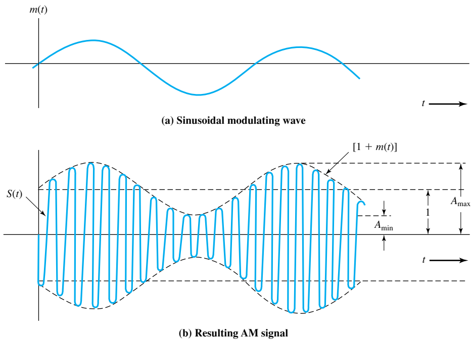
Figure 5.22 Amplitude Modulation
