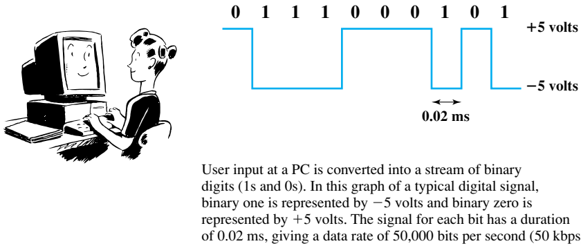
Figure 3.13 Conversion of PC Input to Digital Signal
