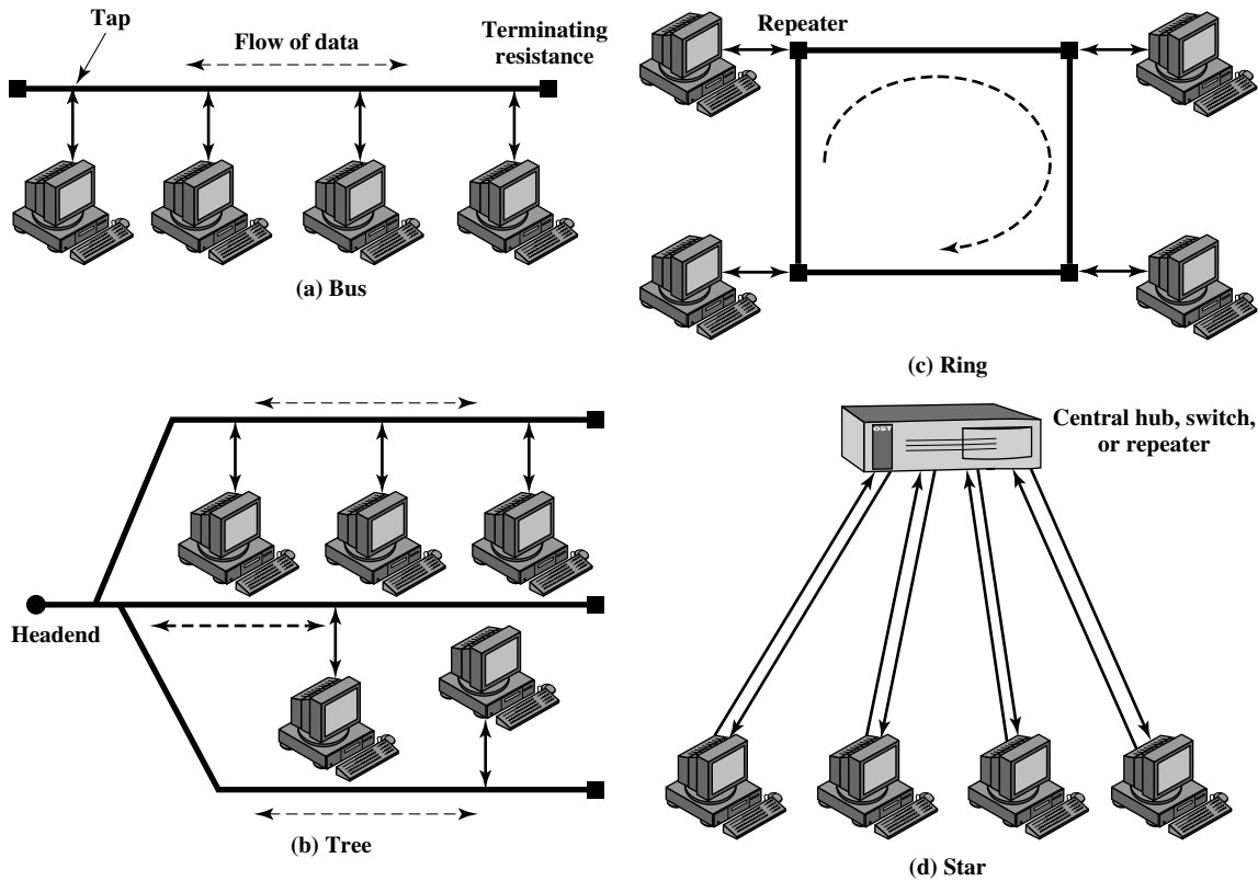
Figure 15.2 LAN Topologies
