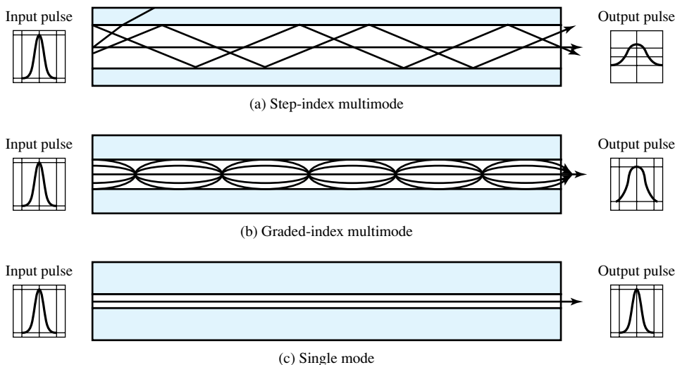
Figure 4.4 Optical Fiber Transmission Modes
