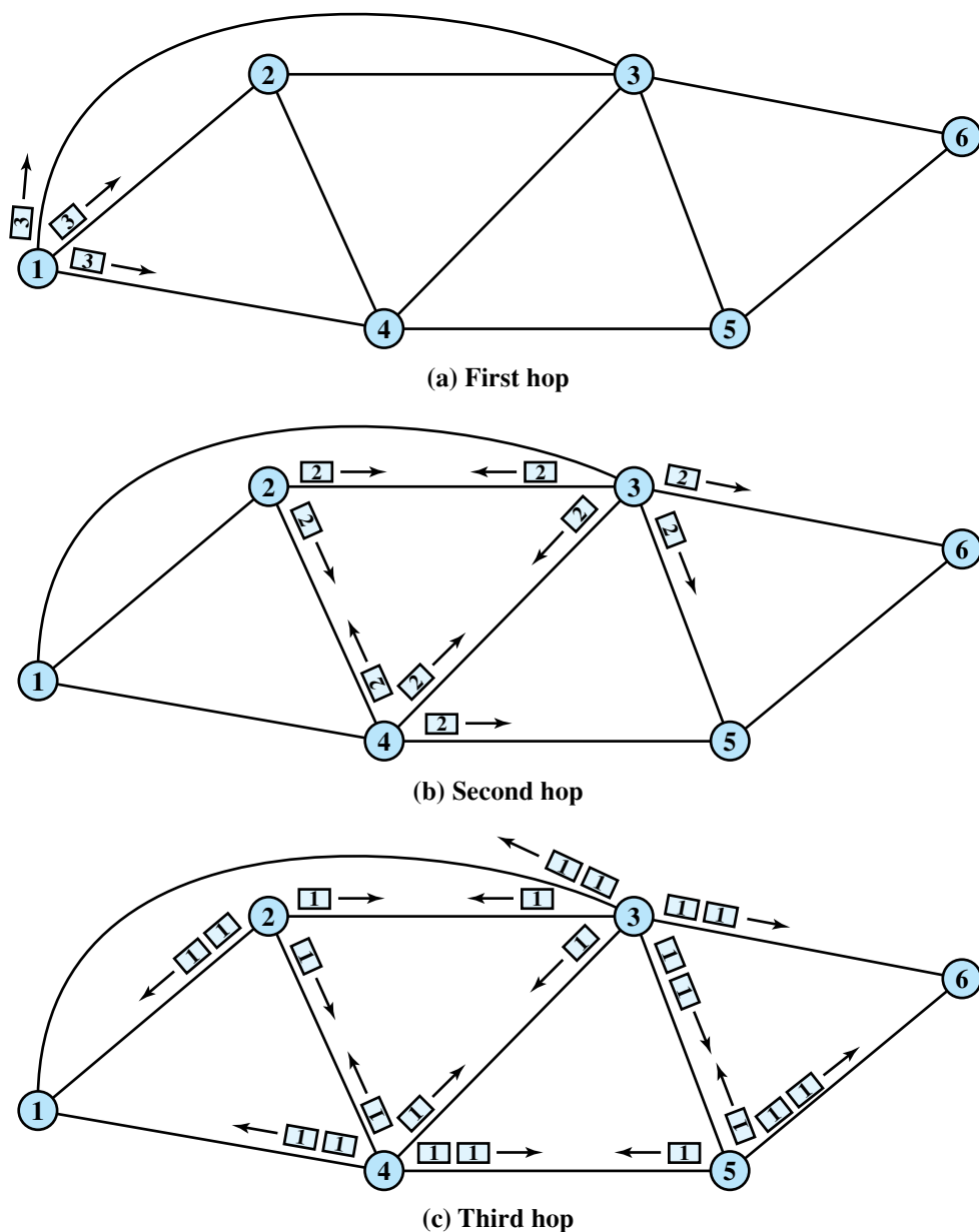
Figure 12.3 Flooding Example (hop count = 3)
