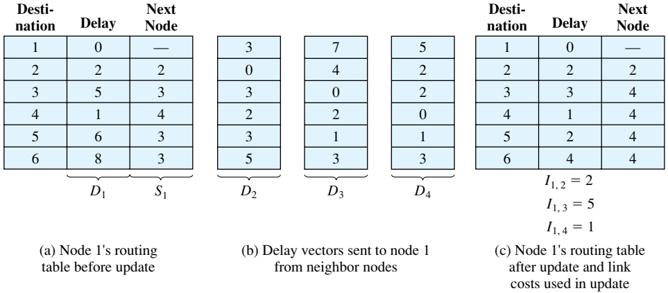
Figure 12.5 Original ARPANET Routing Algorithm
