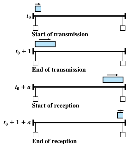
(b) Transmission time = 1; propagation time = a > 1
