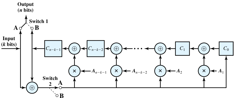
Figure 6.6 General CRC Architecture to Implement Divisor (1 + A_1X + A_2X^2 + \cdots + A_{n-1}X^{n-k-1} + X^{n-k})
