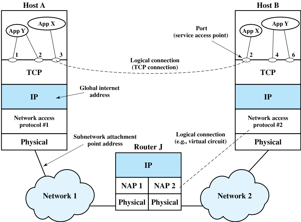
Figure 2.1 TCP/IP Concepts
