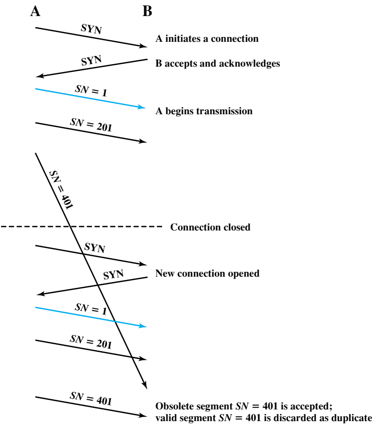
Figure 20.6 The Two-Way Handshake: Problem with Obsolete Data Segment
