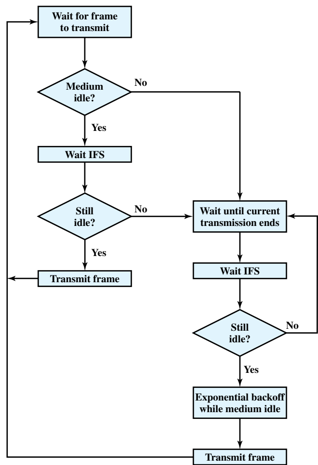
Figure 17.6 IEEE 802.11 Medium Access Control Logic
