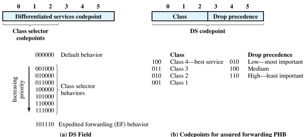
Figure 19.13 DS Field
