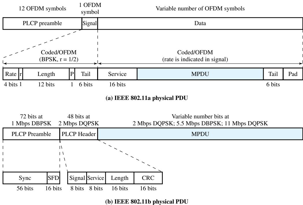
Figure 17.9 IEEE 802 Physical-Level Protocol Data Units
