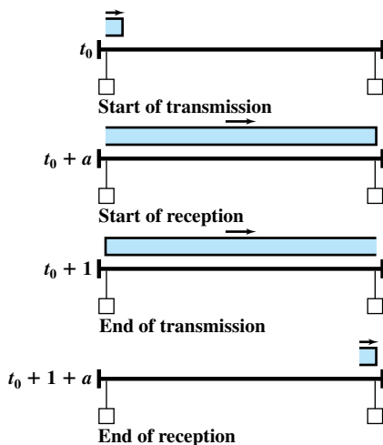
(a) Transmission time = 1; propagation time = a < 1
