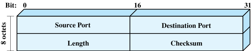
Figure 20.14 UDP Header
