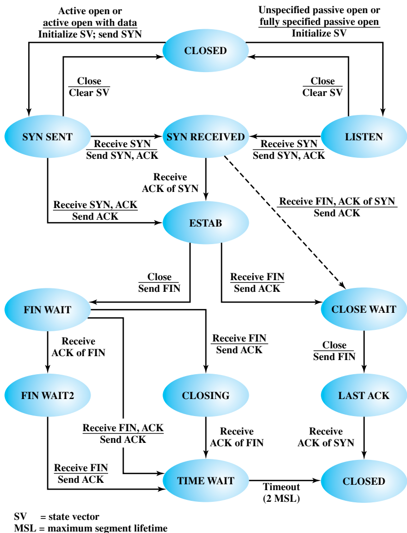
Figure 20.8 TCP Entity State Diagram
