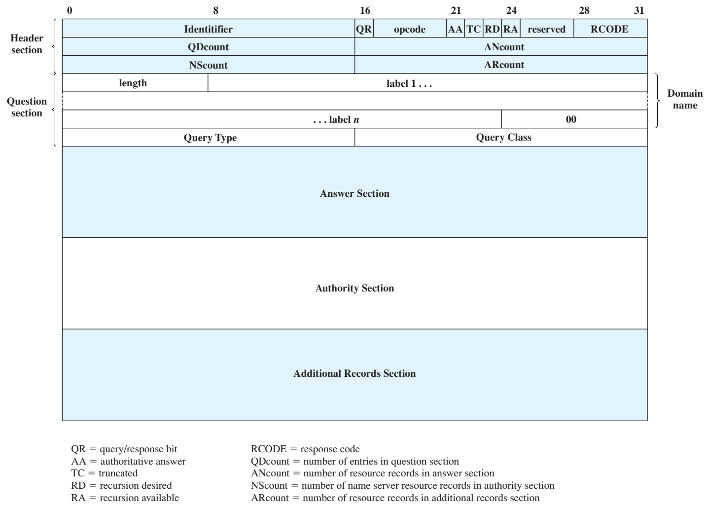
Figure 23.5 DNS Message Format
