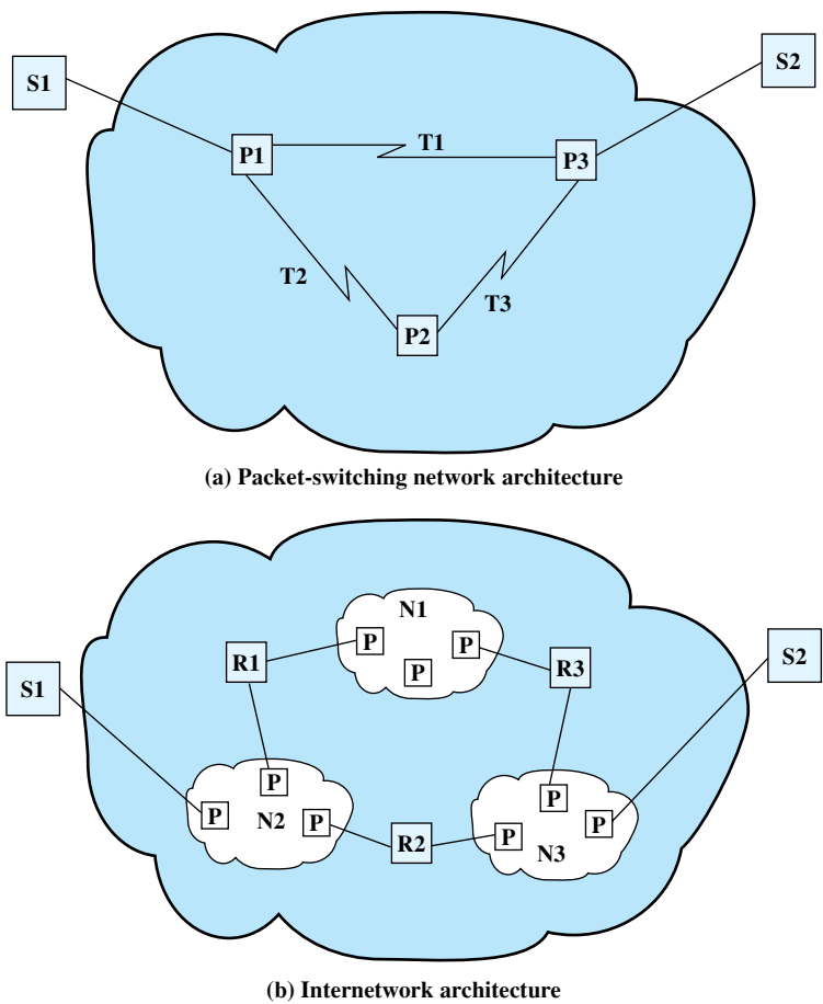
Figure 18.4 The Internet as a Network (based on [HIND83])
