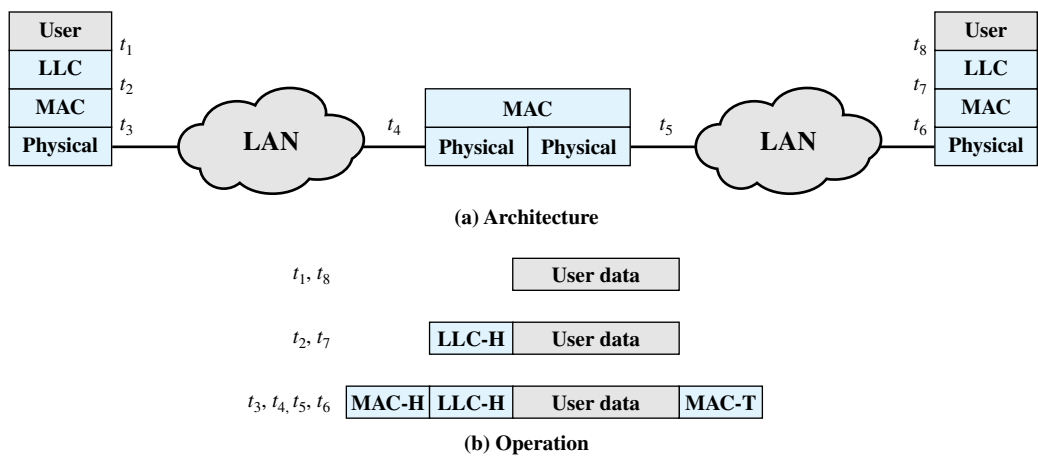
Figure 15.9 Connection of Two LANs by a Bridge
