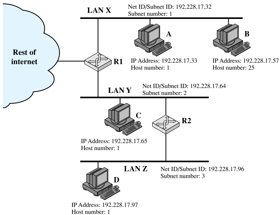
Figure 18.8 Example of Subnetworking
