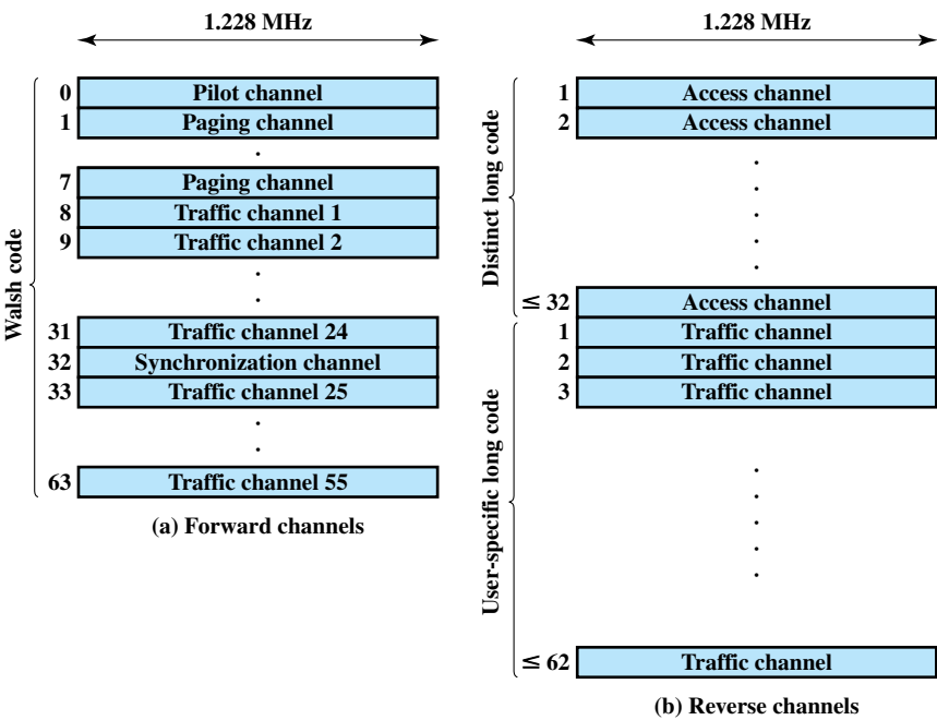
Figure 14.10 IS-95 Channel Structure
