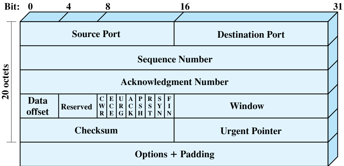
Figure 20.10 TCP Header
