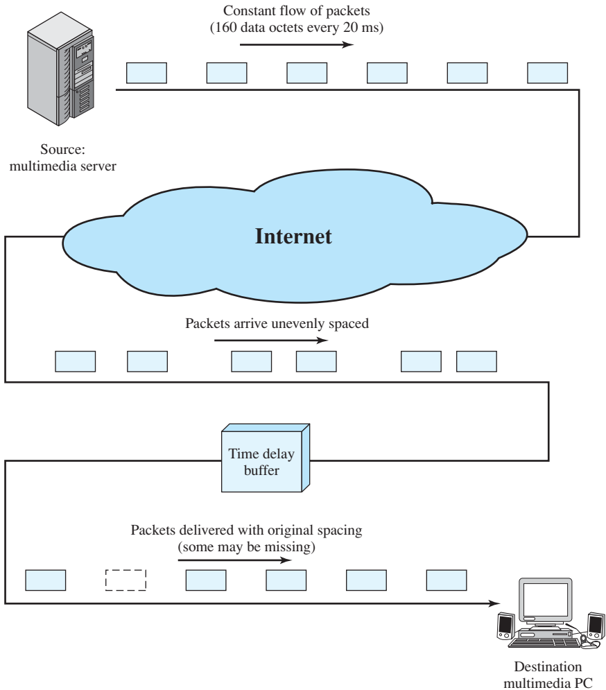
Figure 24.5 Real-Time Traffic
