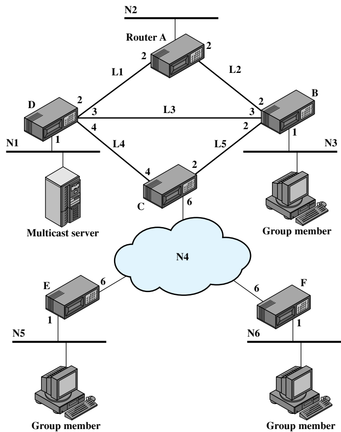
Figure 19.1 Example Configuration
