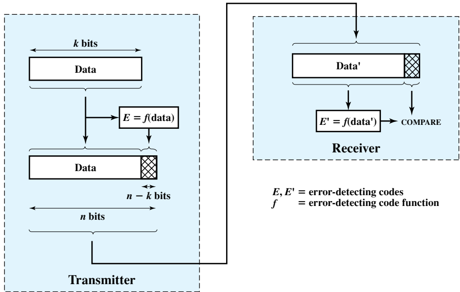
Figure 6.3 Error Detection Process
