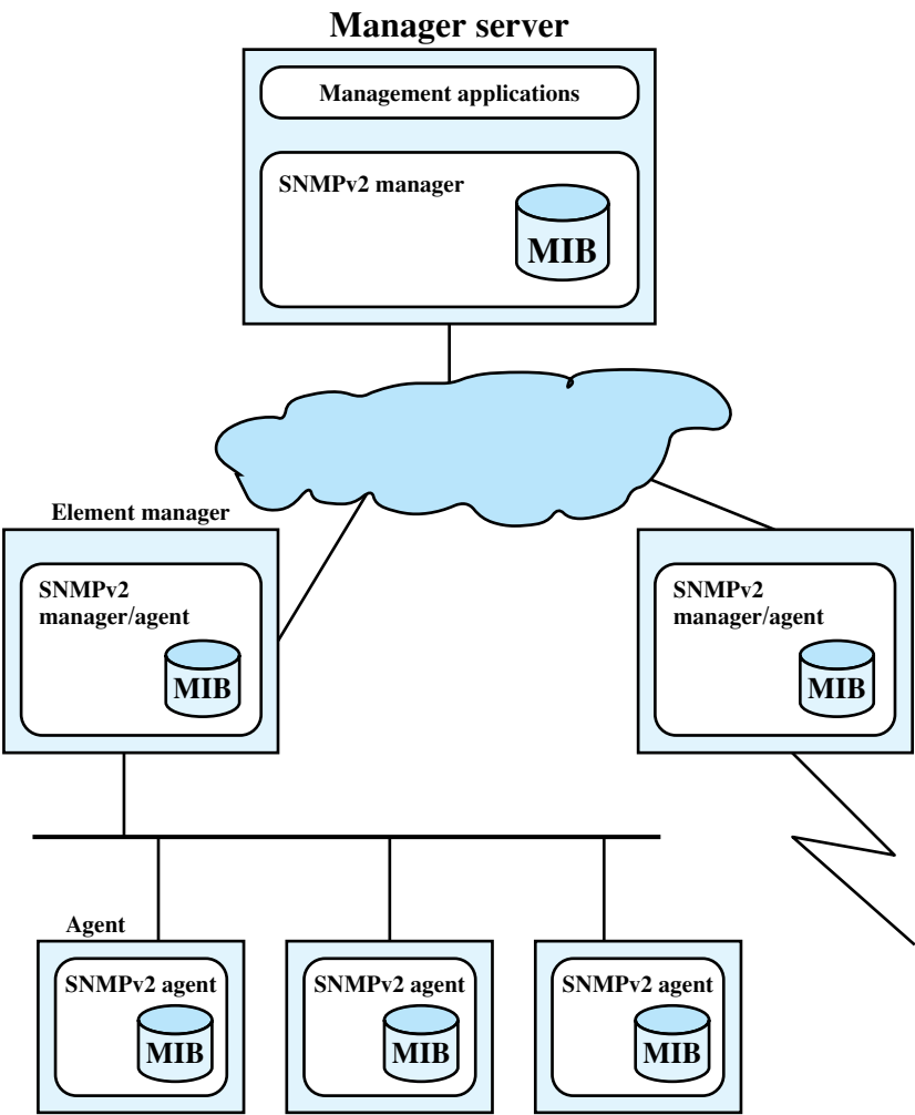
Figure 22.6 SNMPv2-Managed Configuration
