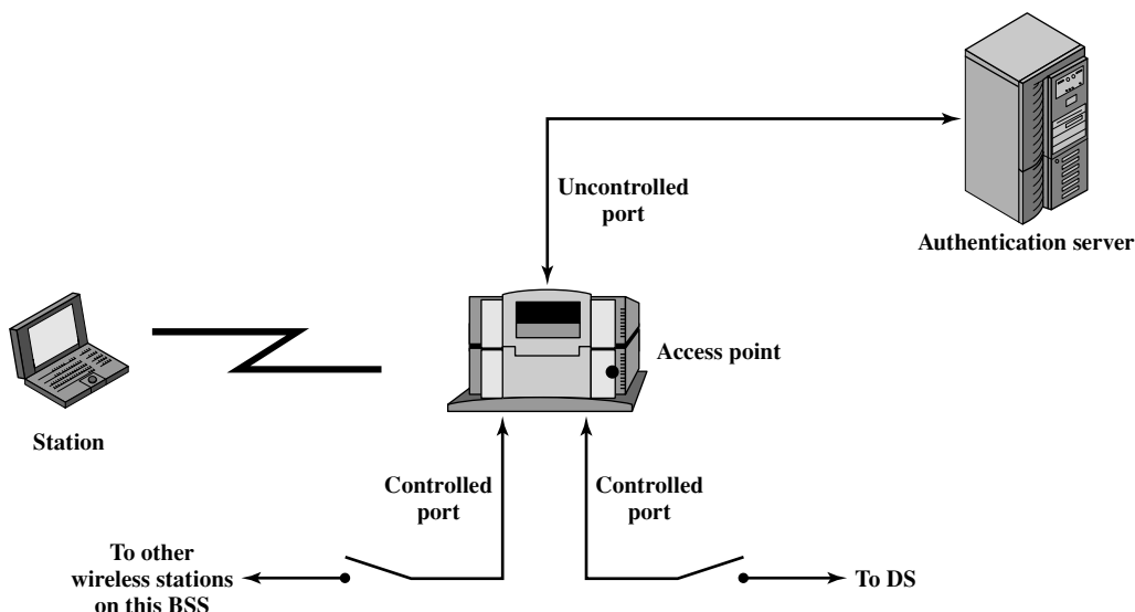
Figure 21.19 802.11i Access Control
