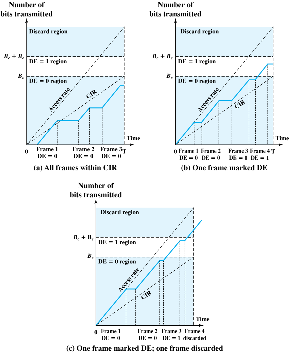
Figure 13.7 Illustration of Relationships among Congestion Parameters
