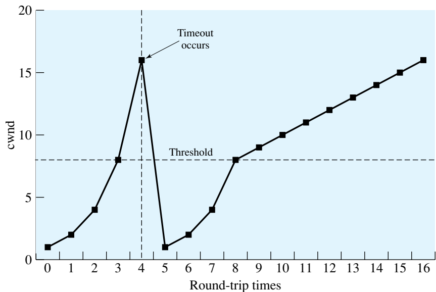
Figure 20.13 Illustration of Slow Start and Congestion Avoidance
