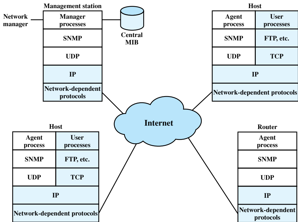
Figure 22.4 SNMPv1 Configuration
