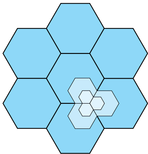
Figure 14.3 Cell Splitting
