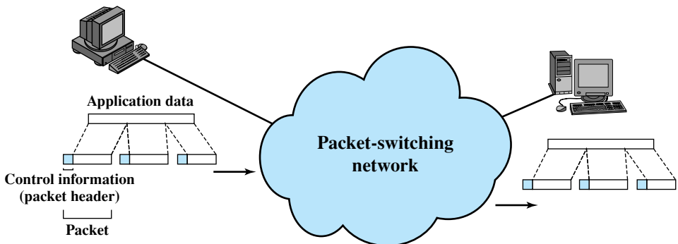
Figure 10.8 The Use of Packets AVAILABLE AT:
