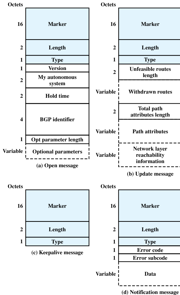
Figure 19.6 BGP Message Formats AVAILABLE AT:
