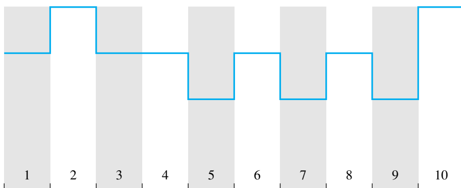
Figure 5.26 A Received Bipolar-AMI Waveform
