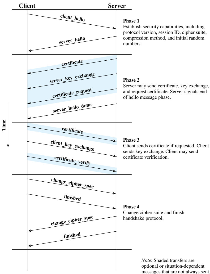
Figure 21.15 Handshake Protocol Action
