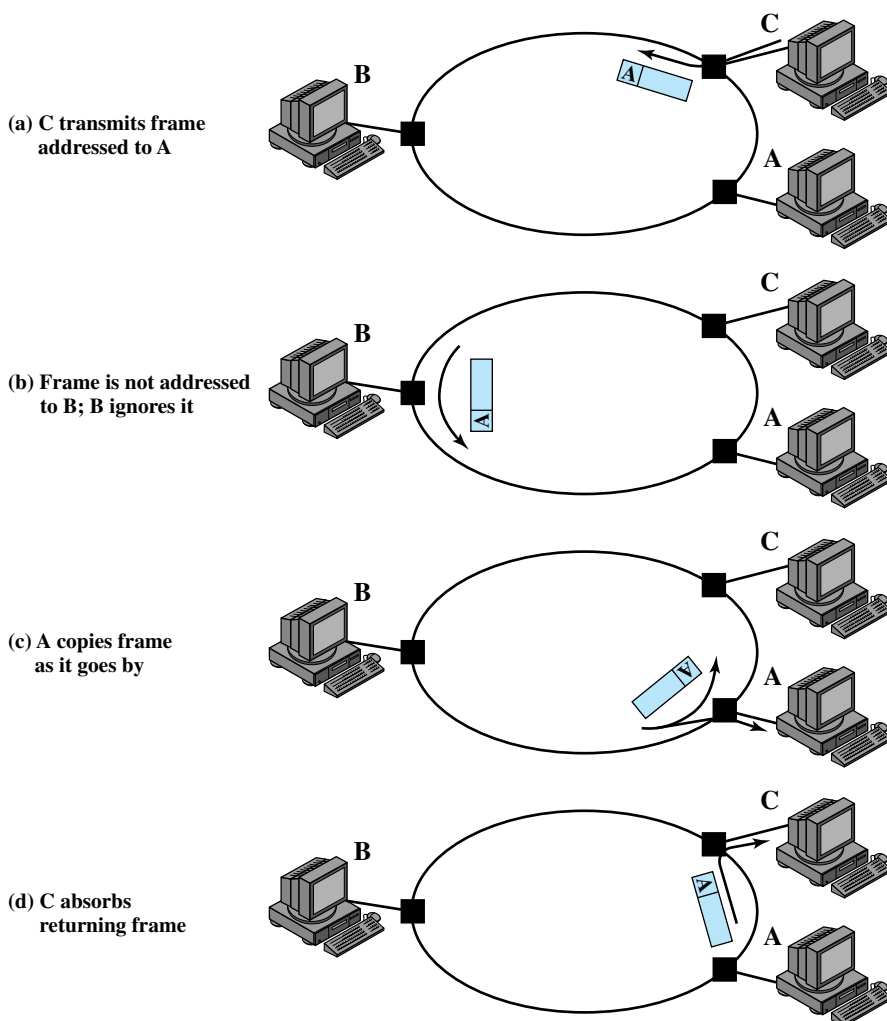
Figure 15.4 Frame Transmission on a Ring LAN
