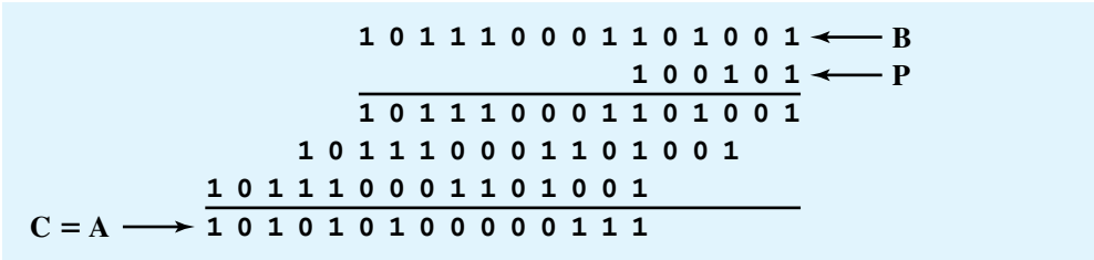
(b) Descrambling
