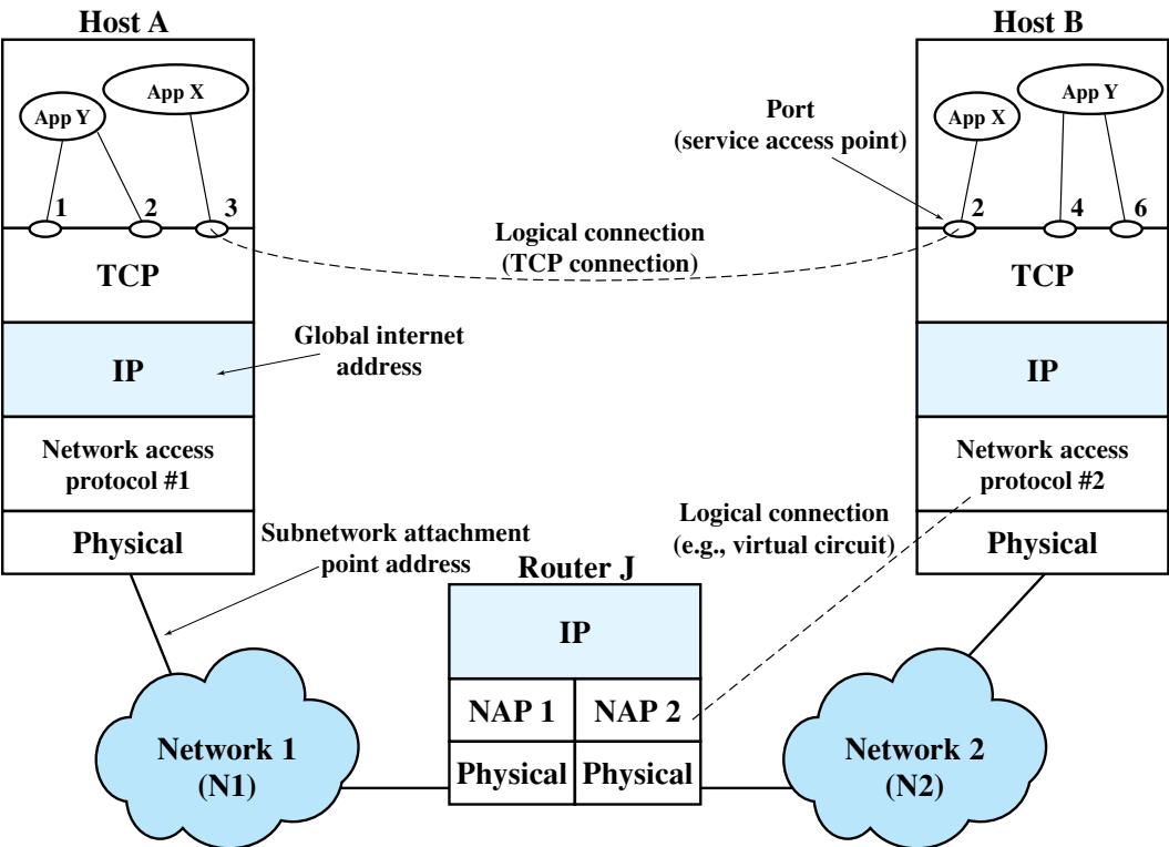
Figure 18.2 TCP/IP Concepts
