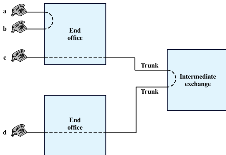
Figure 10.3 Circuit Establishment
