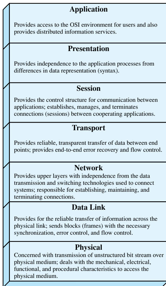
Figure 2.6 The OSI Layers
