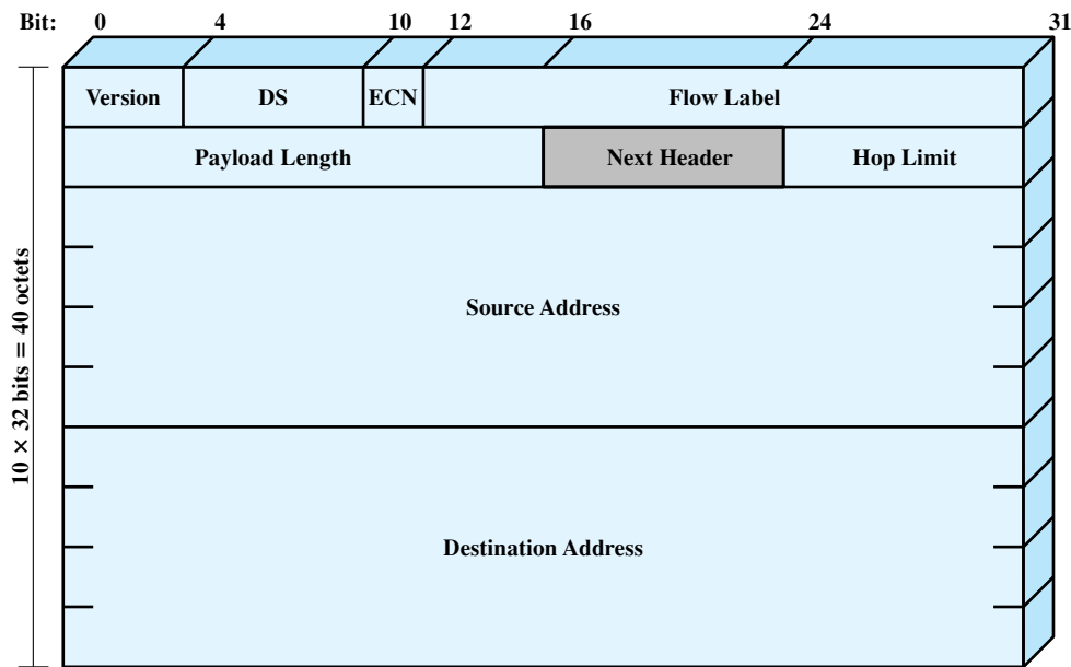
Figure 18.11 IPv6 Header
