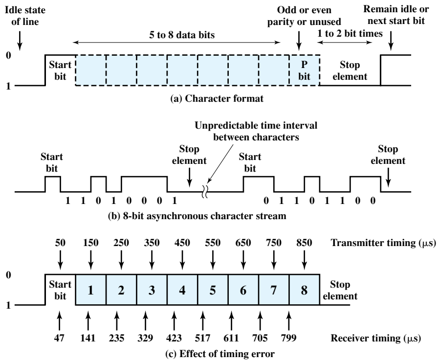
Figure 6.1 Asynchronous Transmission
