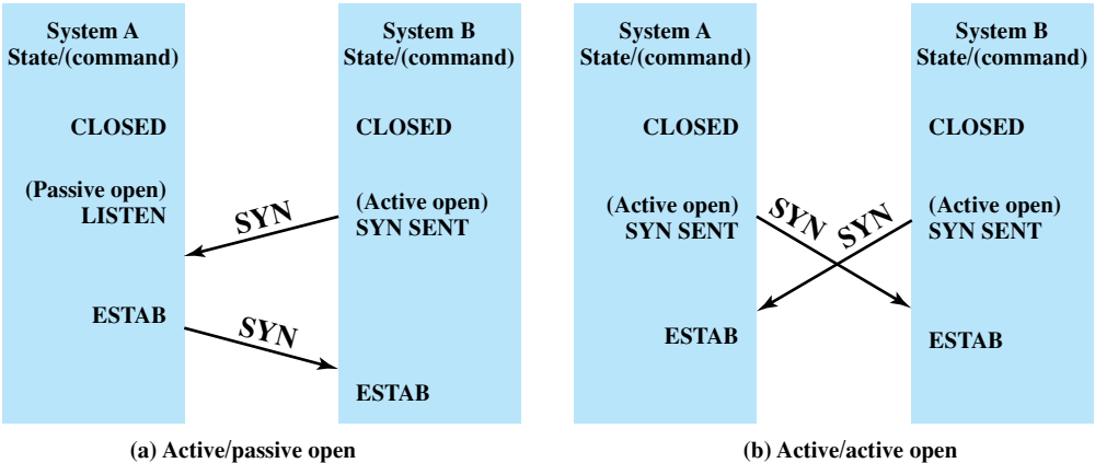
Figure 20.4 Connection Establishment Scenarios
