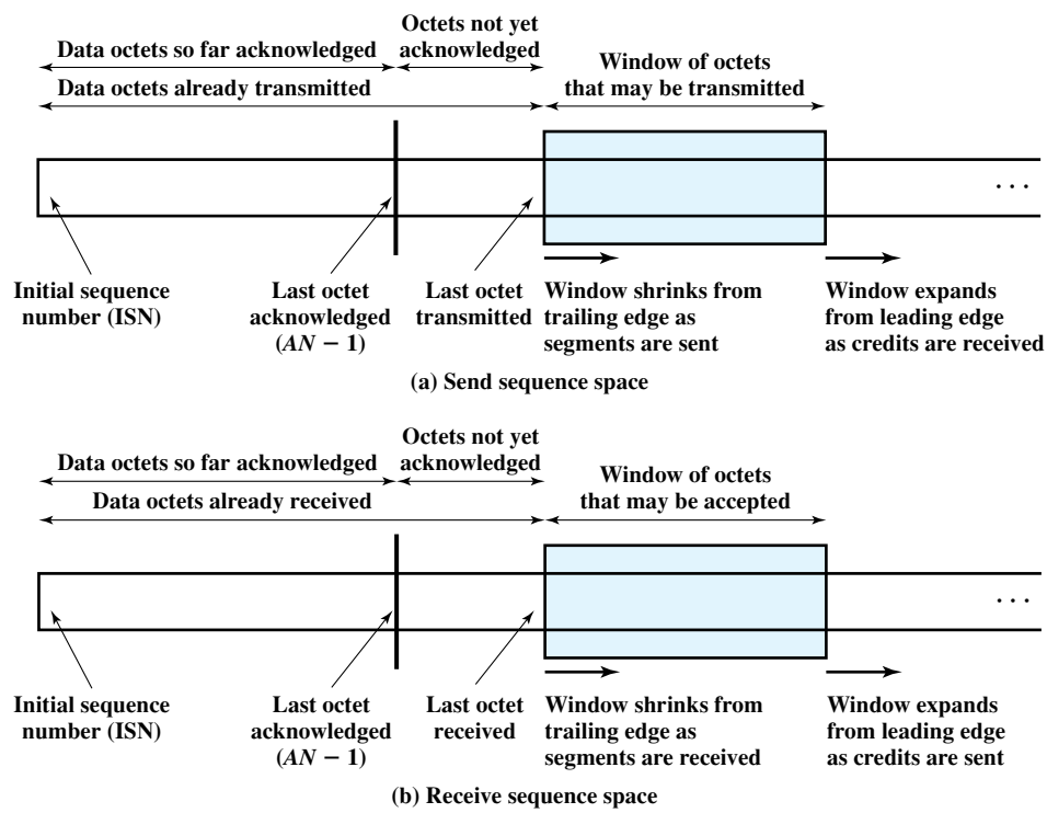
Figure 20.2 Sending and Receiving Flow Control Perspectives
