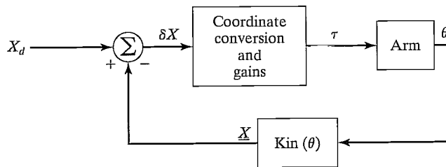
FIGURE 10.11: The concept of a Cartesian-based control scheme.
